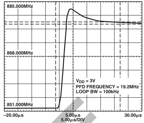
TPC 4. PLL Settling Time, 852 MHz to 878 MHz, 23 \mu s ( \pm 400 kHz)
