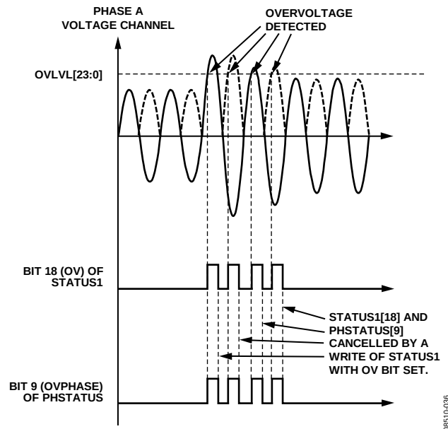
Figure 52. Overvoltage Detection
