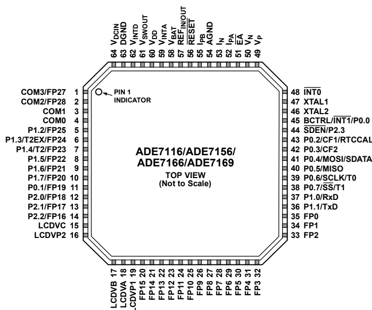
Figure 10. Pin Configuration for the ADE7116/ADE7156/ADE7166/ADE7169
