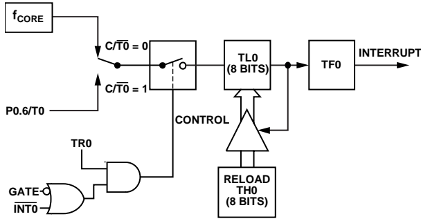
Figure 100. Timer/Counter 0, Mode 2
