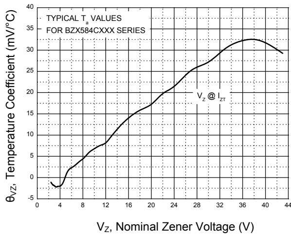
Figure 3. Temperature Coefficients
