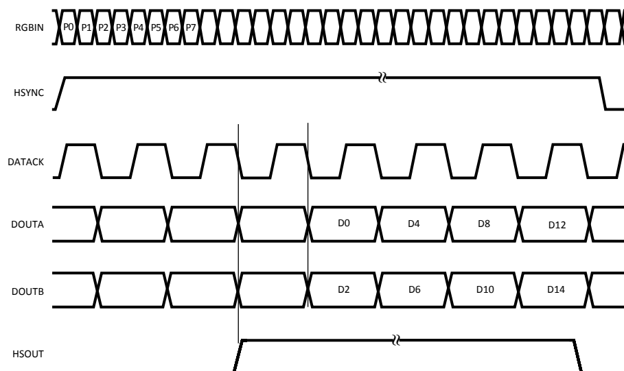
Figure 7. Dual Channel Mode - Interleaved Outputs - 2 Pixels/Clock - Odd Pixels
