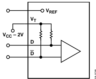
CONNECT V_T TO V_{CC} - 2V .
