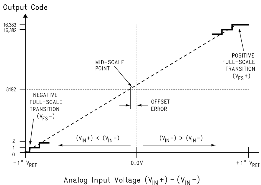
Figure 5. Transfer Characteristic
