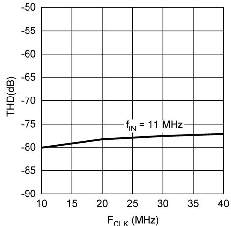
Figure 19. THD vs. f_CLK
