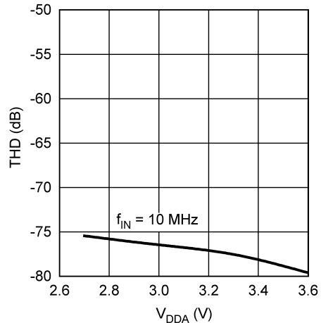
Figure 17. THD vs. V_DDA
