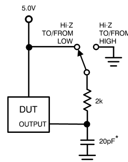
Figure 21. t_{EN}, t_{DIS} Test Circuit
