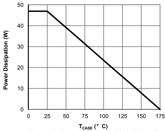
Figure 11B: Power De-rating for TO220F (Note F)
