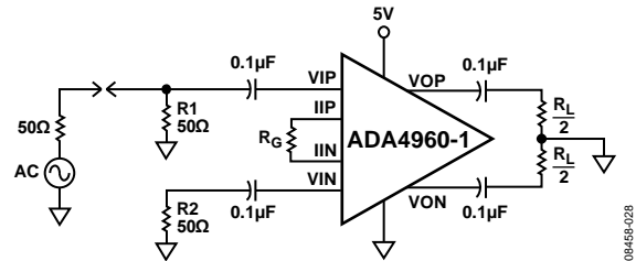
Figure 32. Single-Ended-Input-to-Differential-Output Configuration
