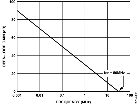
Figure 54. ADA4941-1 Op Amp Open-Loop Gain vs. Frequency
