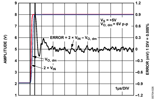
Figure 28. Settling Time (0.005%), V_S = +5 V
