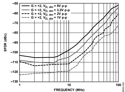
Figure 3. SFDR vs. Frequency and Output Voltage
