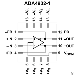
Figure 1. ADA4932-1
