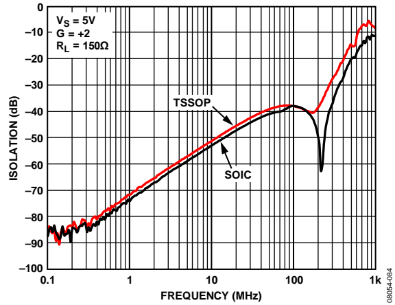
Figure 46. Forward Isolation vs. Frequency (ADA4891-3 Only)
