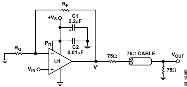
Figure 45. Video Amplifier
