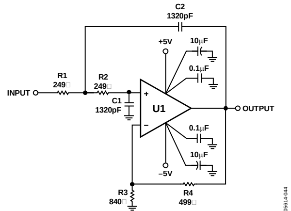
Figure 49. Two-Pole 500 kHz Reconstruction Filter Schematic
