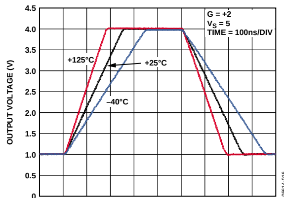
Figure 27. Slew Rate vs. Temperature
