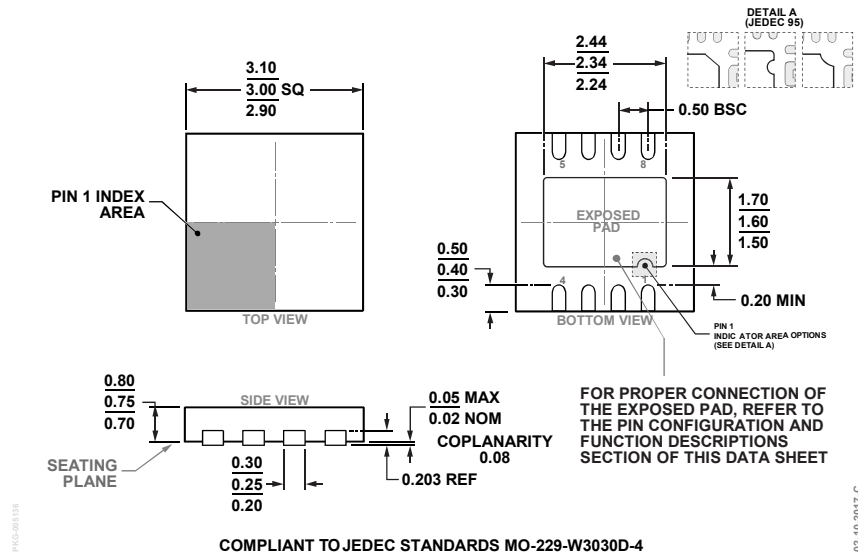
COMPLIANT TO JEDEC STANDARDS MO-229-W3030D-4 Figure 55. 8-Lead Lead Frame Chip Scale Package [LFCS] 3 mm x 3 mm Body and 0.75 mm Package Height (CP-8-11) Dimensions shown in millimeters
