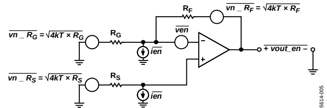
Figure 40. Noise Sources in Typical Connection
