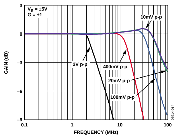
Figure 11. Frequency Response for Various V_{OUT}
