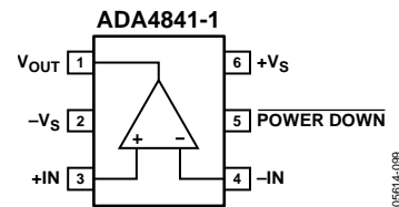
Figure 2. 6-Lead SOT-23 (RJ)
