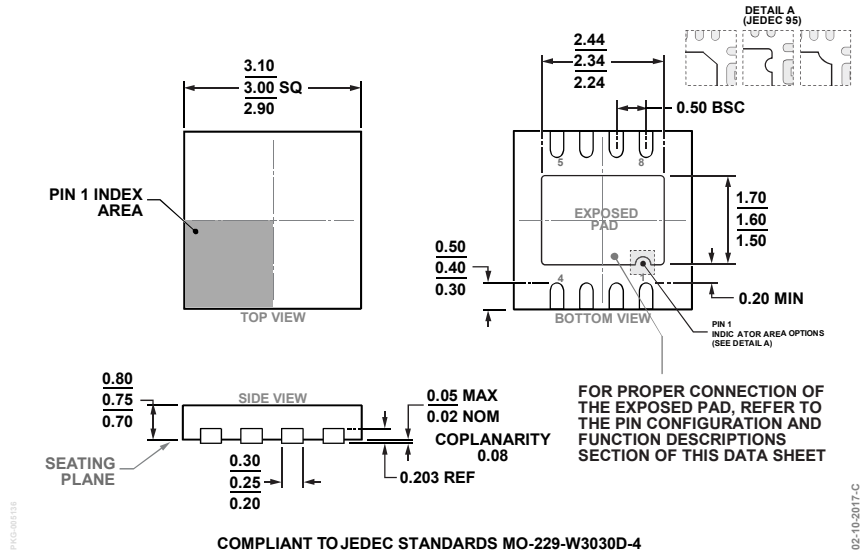
COMPLIANT TO JEDEC STANDARDS MO-229-W3030D-4 Figure 55. 8-Lead Lead Frame Chip Scale Package [LFCSP] 3 mm × 3 mm Body and 0.75 mm Package Height (CP-8-11) Dimensions shown in millimeters
