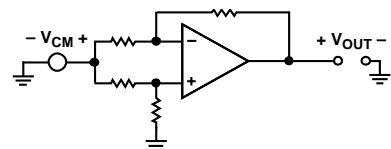
Figure 44. Common-Range Subtractor
