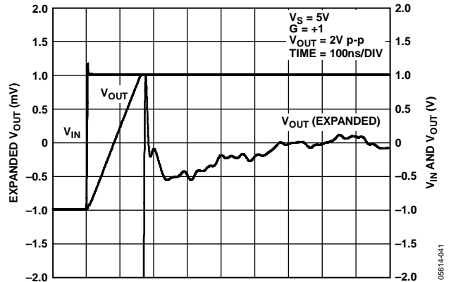
Figure 28. Settling Time
