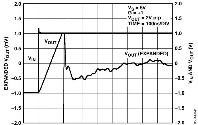
Figure 28. Settling Time
