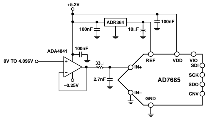
Figure 50. ADC Driver Schematic Rev. G | Page 17 of 20
