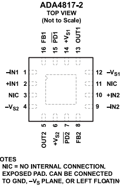
Figure 7. ADA4817-2 Pin Configuration (16-Lead LFCSP)
