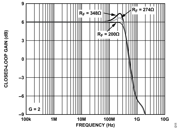
Figure 13. Small Signal Frequency Response for Various R_F
