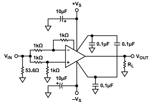
Figure 51. Common-Mode Rejection
