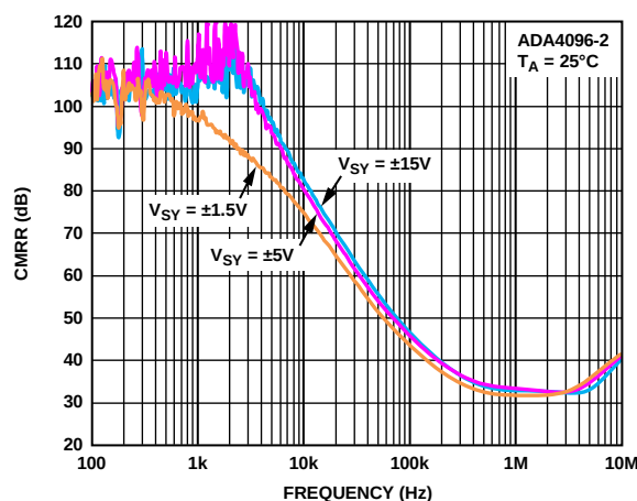
Figure 49. CMRR vs. Frequency
