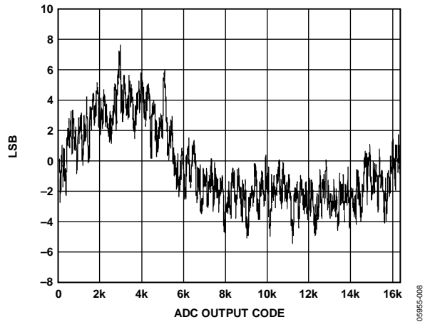
Figure 7. Integral Nonlinearity
