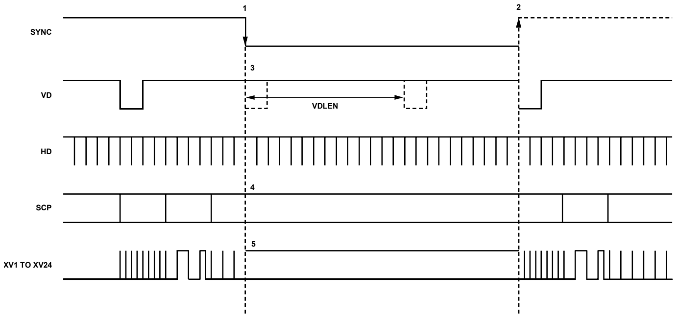
Figure 80. Enhanced SYNC Mode 2 with Vertical Signals Held at VTP Start Value
