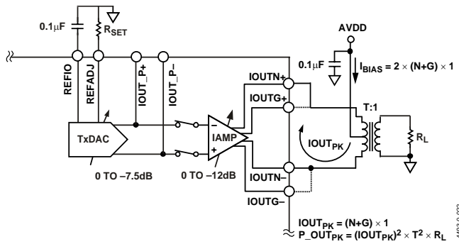
Figure 64. Current-Mode Operation
