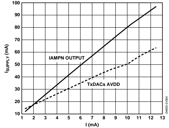
Figure 66. Current Consumption of TxDAC and IAMP in Current-Mode Operation with IOUTN Only (Default IAMP Settings)
