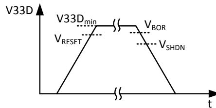
Figure 30. Reset and Brownout Thresholds
