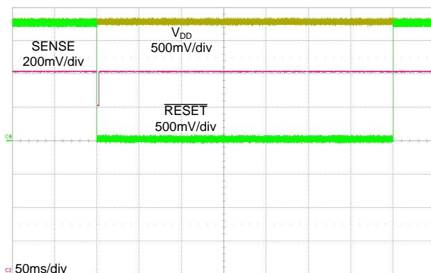
Figure 38. Typical RESET Delay Timing
