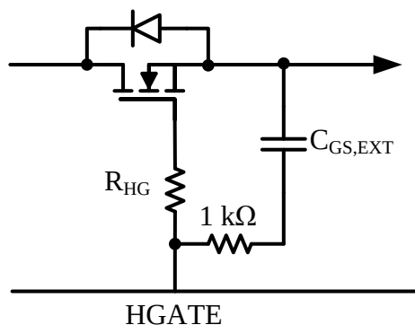
Figure 32. Ensuring Stability
