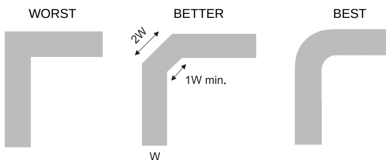
Figure 10. Trace Example
