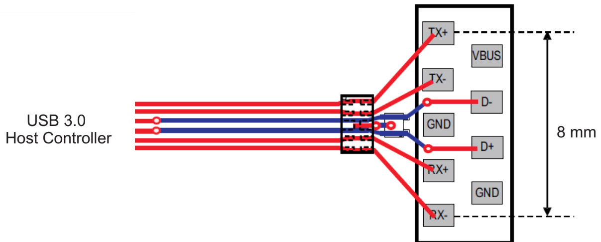
Figure 21. Flow-Through Routing
