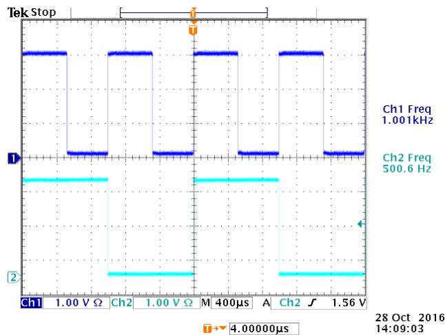
Figure 8. Frequency Division
