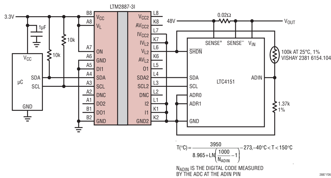
Figure 26. Isolated I 2 C Voltage, Current and Temperature Power Supply Monitor
