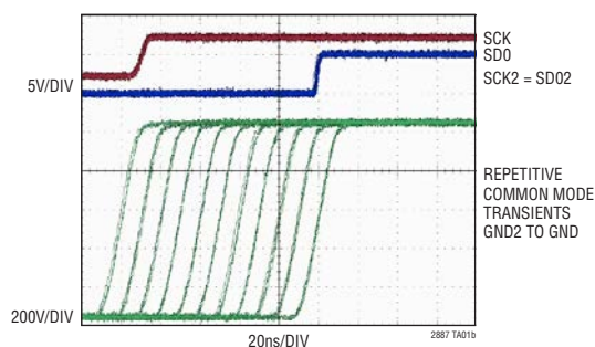
LTM2887 Operating Through 50kV/μs CM Transients
