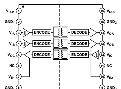
Figure 2. ADuM1301 Functional Block Diagram
