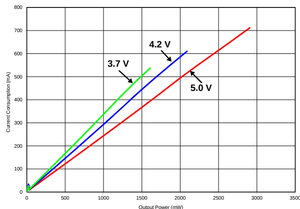
Figure 55. Supply Current vs. Output Power - FHD Mode R_L = 4 \Omega + 33 \mu\text{H}
