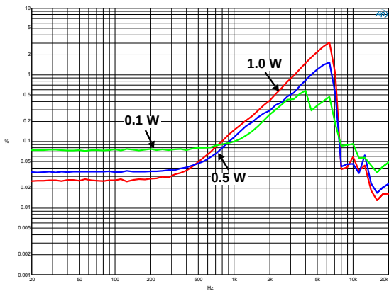
Figure 22. THD+N vs. Frequency - FSD Mode V_{BATT} = 5.0 \text{ V}
