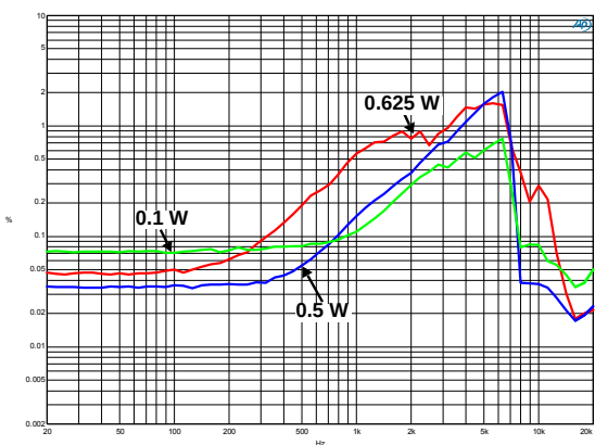
Figure 24. THD+N vs. Frequency - FSD Mode V_{BATT} = 3.7 \text{ V}
