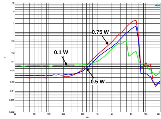
Figure 23. THD+N vs. Frequency - FSD Mode V_{BATT} = 4.2 \text{ V}
