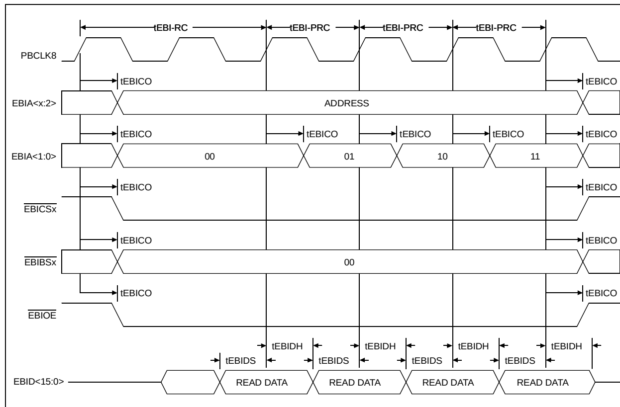
FIGURE 37-28: EBI PAGE READ TIMING
