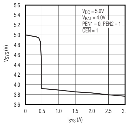
SYS OUTPUT VOLTAGE vs. SYS OUTPUT CURRENT (500mA USB)
