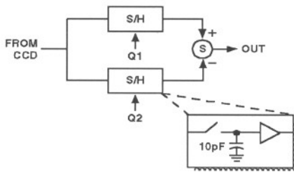
Figure 24. CDS Block Diagram
