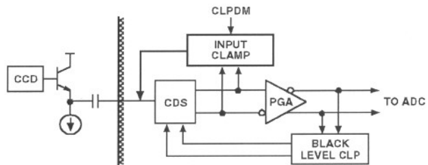
Figure 30. Input Clamp
