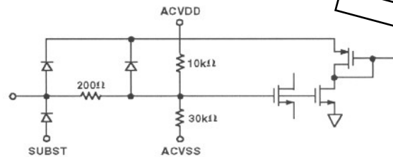
Figure 10. Pin 32 (CLPBYP)
