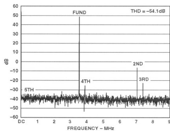
Figure 22. ADC-MODE THD at 18 MHz ( f_N = 3.54 MHz at -3 dB)
