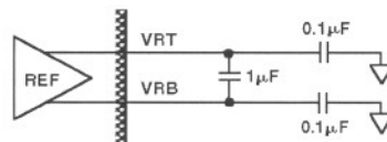
Figure 31. Reference Decoupling
