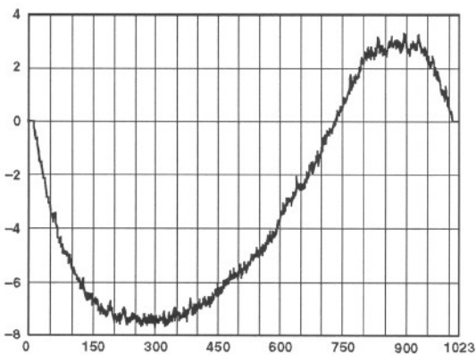
Figure 19. CCD-MODE INL at 18 MHz
