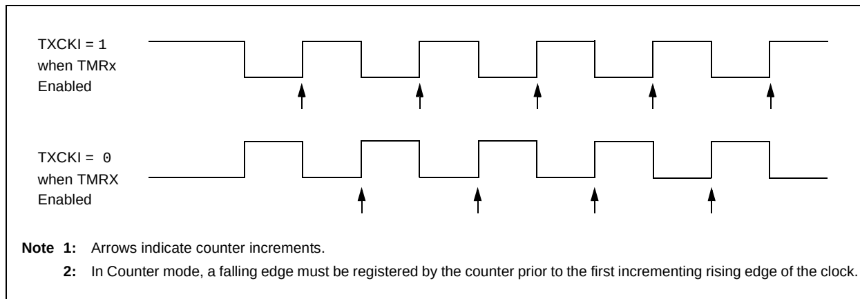
FIGURE 12-3: TIMER1/3/5 INCREMENTING EDGE
