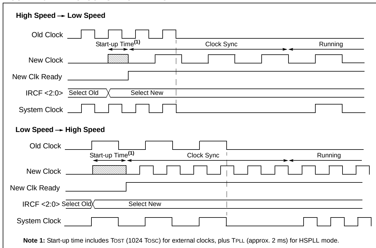
FIGURE 2-9: CLOCK SWITCH TIMING
