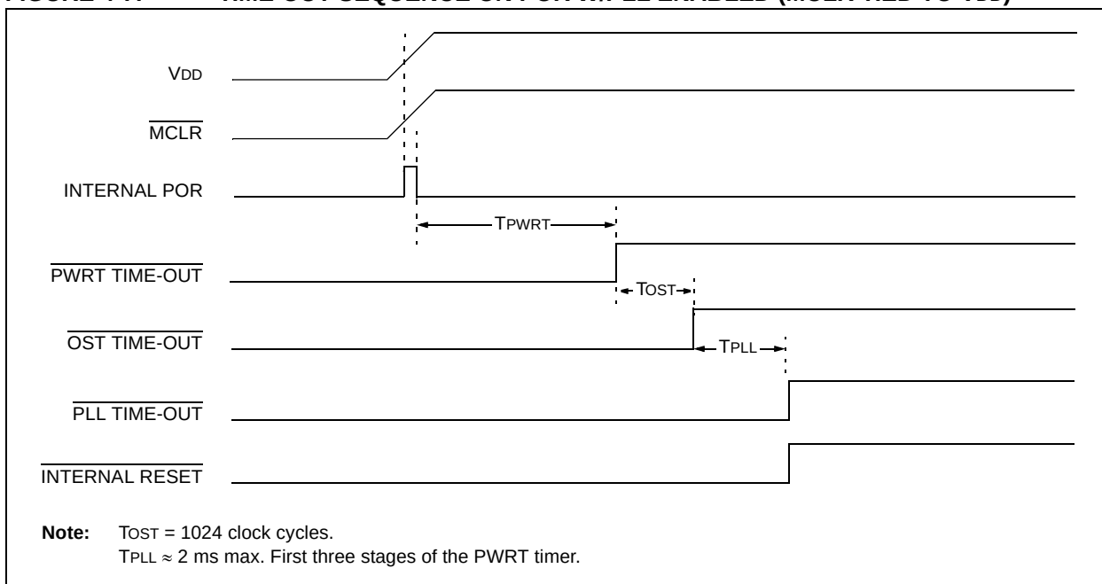
FIGURE 4-7: TIME-OUT SEQUENCE ON POR W/PLL ENABLED (MCLR TIED TO V DD )
