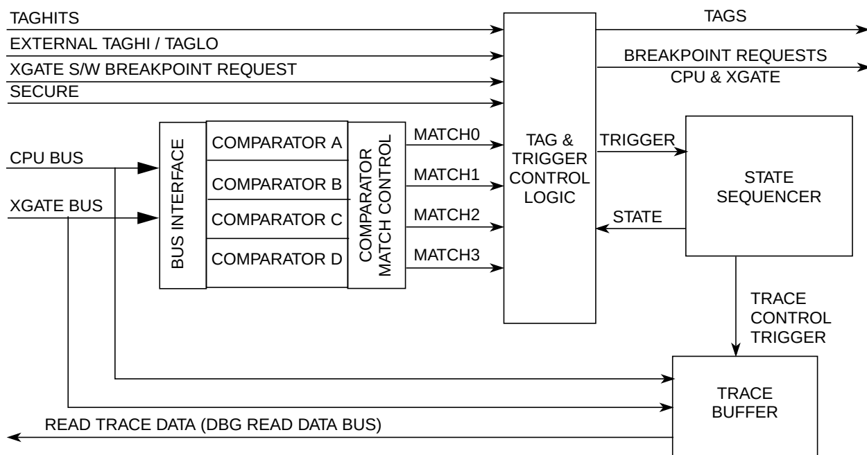
Figure 19-22. DBG Overview
