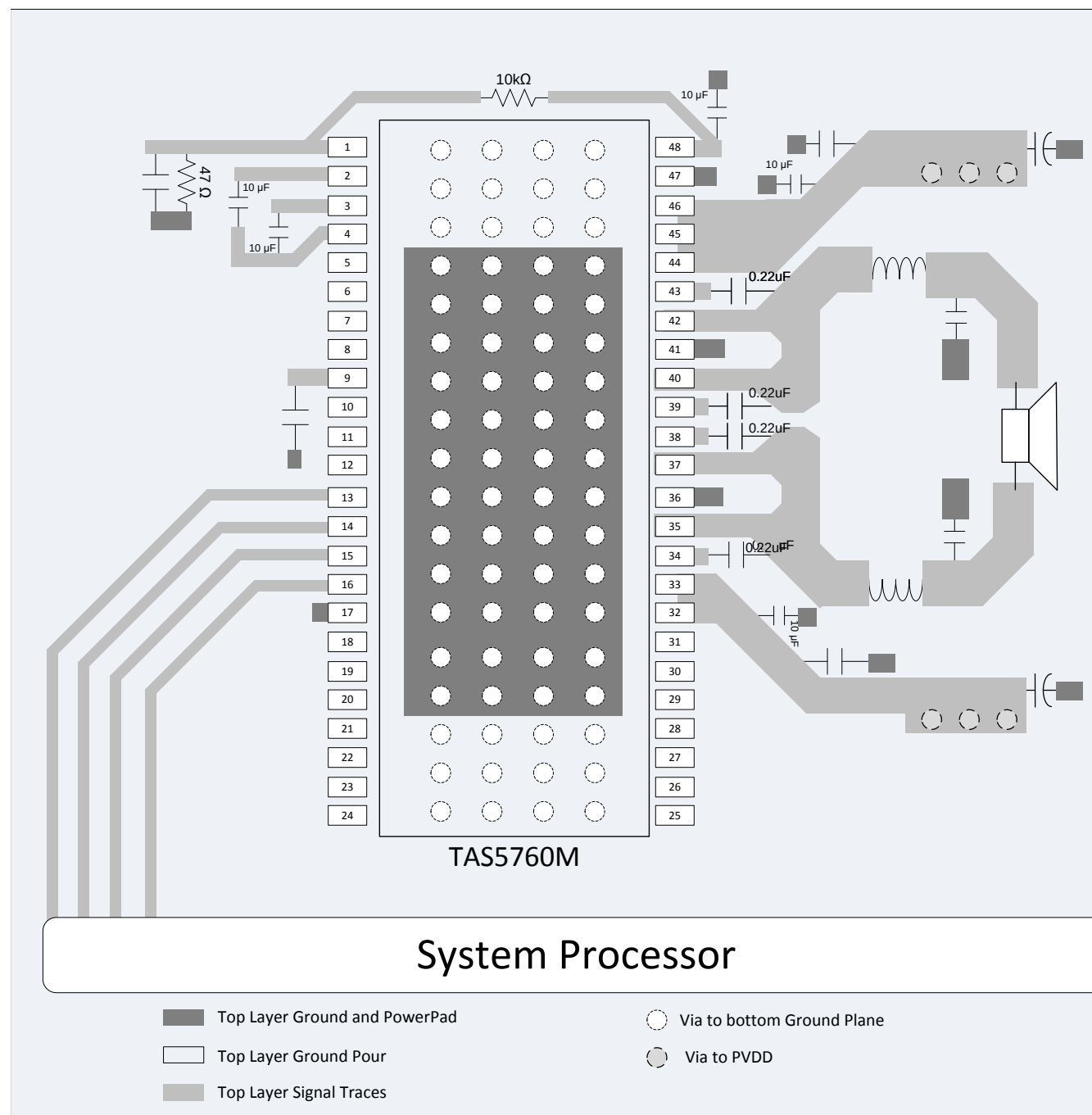
Figure 72. DCA Package PBTL Configuration
