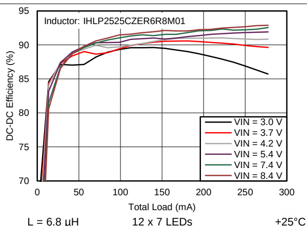
Figure 4. Boost Efficiency
