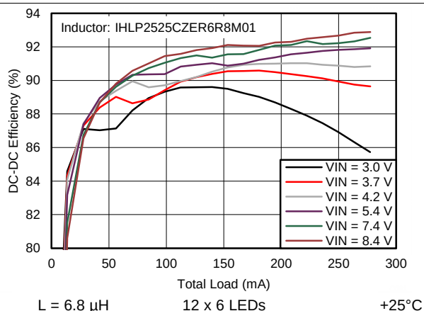
Figure 2. Boost Efficiency
