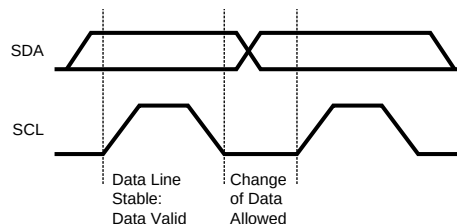
Figure 37. Bit Transfer
