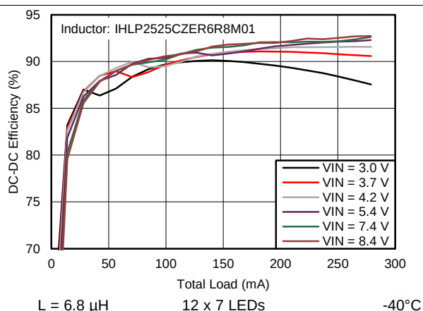
Figure 6. Boost Efficiency
