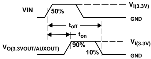
Turn On/Off Time (3.3VOUT/AUXOUT)
