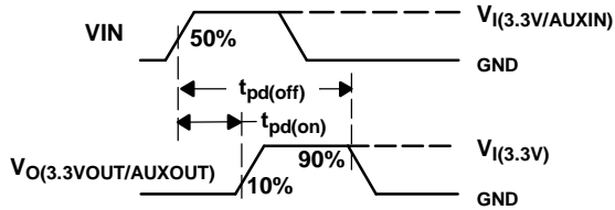
Propagation Delay (3.3VOUT/AUXOUT)
