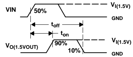
Turn On/Off Time (1.5VOUT)
