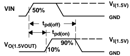
Propagation Delay (1.5VOUT)
