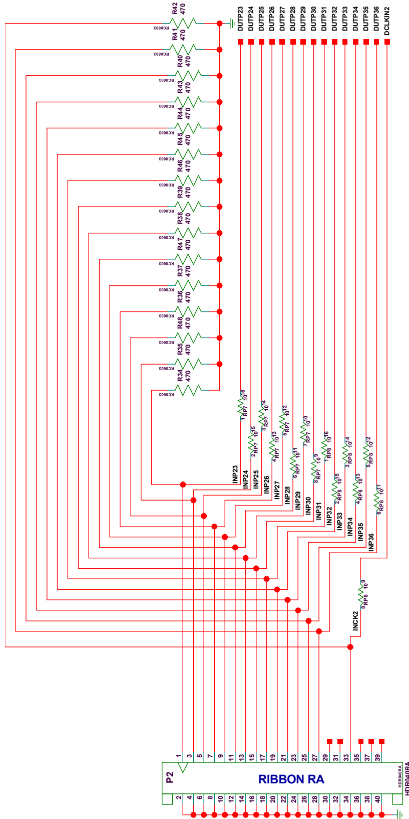
Figure 90. Digital Input Signaling (2)
