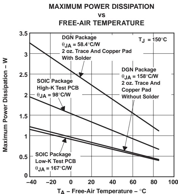
Figure 71. Maximum Power Dissipation vs Free-Air Temperature
