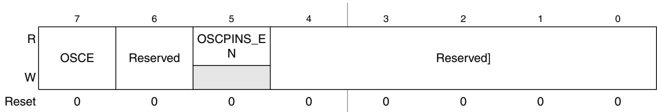
Figure 10-27. S12CPMU Oscillator Register (CPMUOSC)
