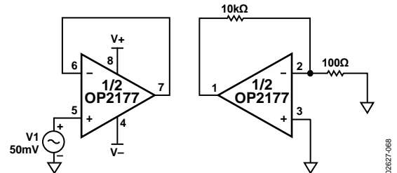
Figure 68. Channel Separation Test Circuit
