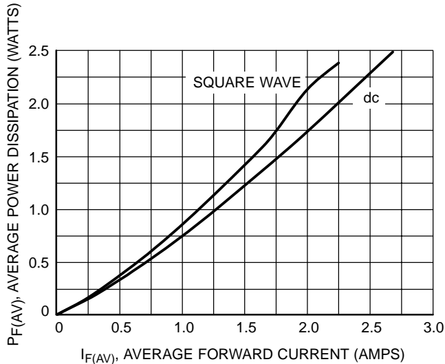
Figure 6. Power Dissipation
