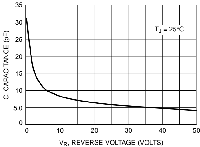
Figure 8. Maximum Capacitance
