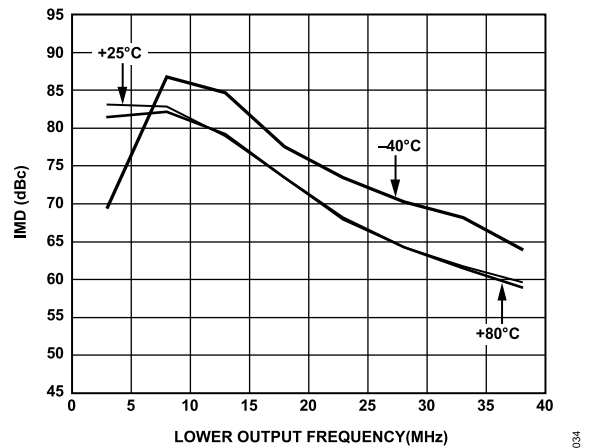
Figure 37. Dual-Tone IMD vs. Lower f_{OUT} and Temperature at 80 MSPS, I_{OUTFS} = 2 mA and 0 dBFS
