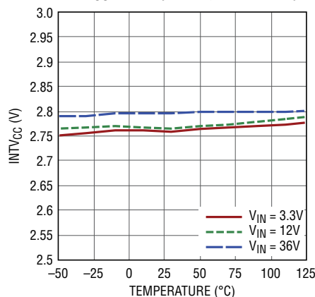
INTV CC UVLO (Falling Threshold)
