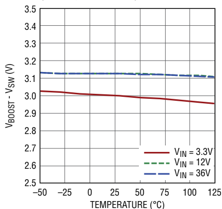
V BOOST - V SW UVLO (Falling Threshold)
