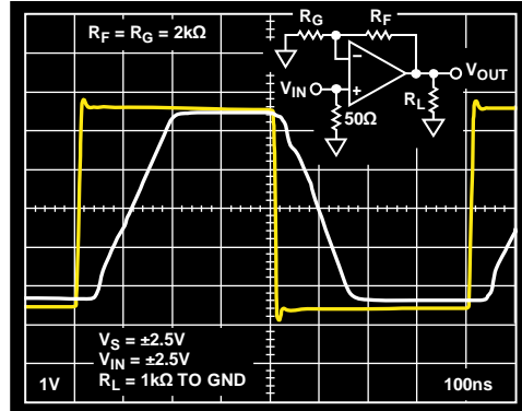
Figure 45. Overdrive Recovery
